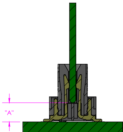
FIGURE 1 MEC8 MATED
