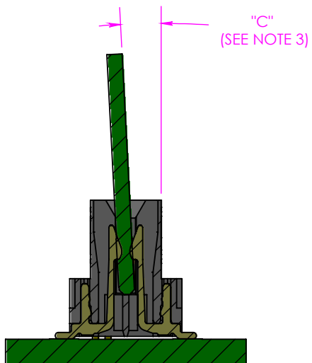
FIGURE 4 MEC8 MATED
